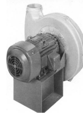
Arrangement 4 (Foot mounted motor)
