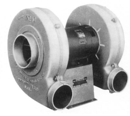
Arrangement 4D (Double blower unit)
